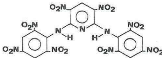
2,6-bis(picrylamino)-3,5-dinitropyridine
